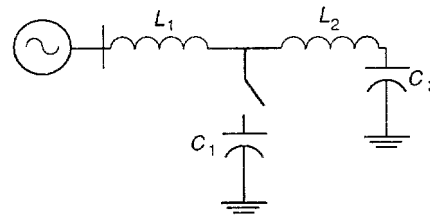
Figure 11—Equivalent circuit for magnification condition
